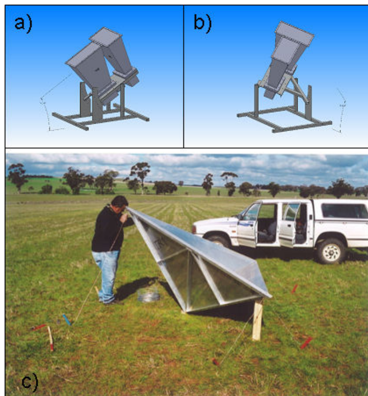
Figure 5-11. Polarimetric Active Radar Calibrators #1 and #2 (a), #3 (b) and Passive Radar Calibrator (c)
