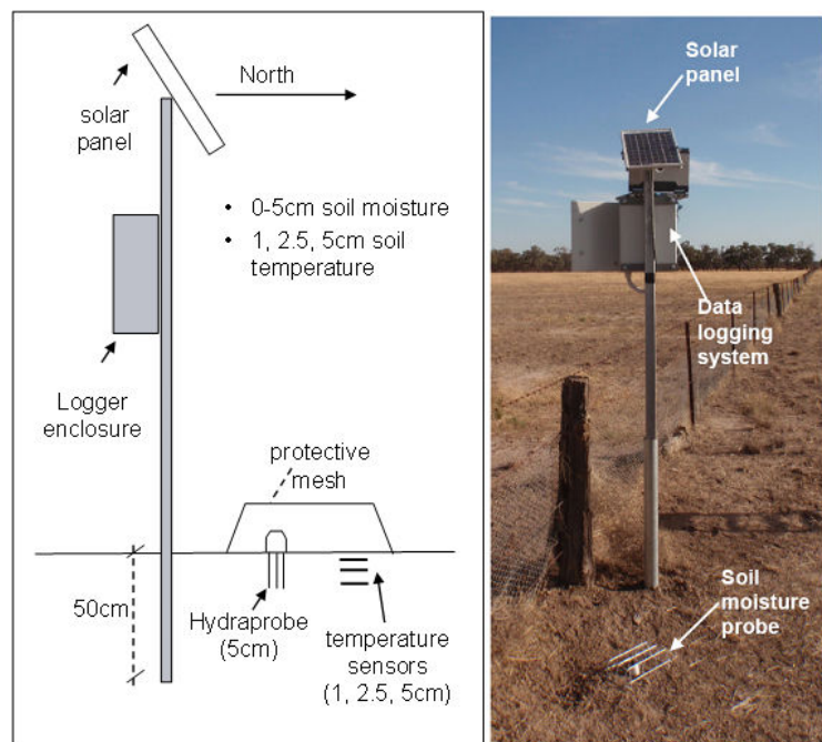
Figure 4-7. Schematic layout of the additional SMAPEX monitoring site and photo of one site.
