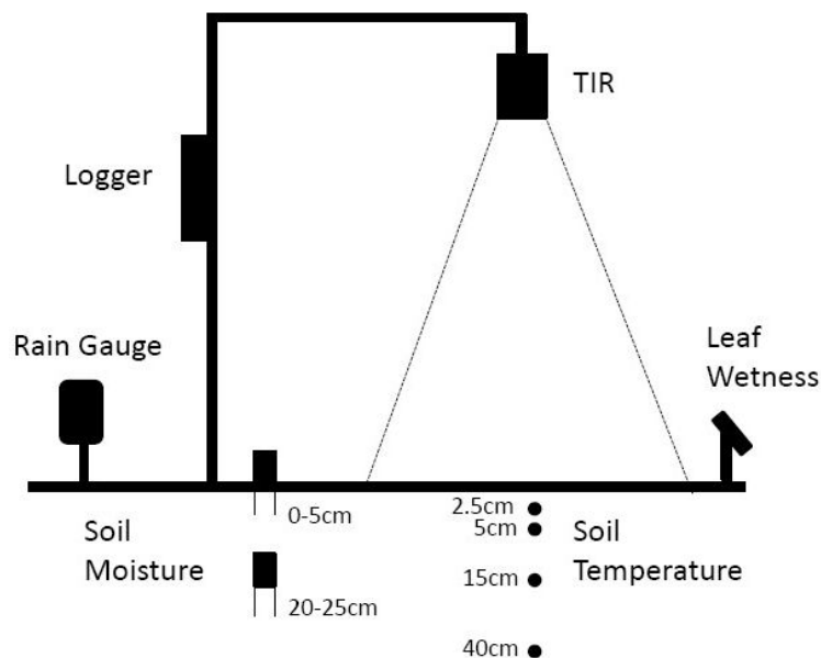
Figure 6-1. Schematic of the temporary monitoring station.
